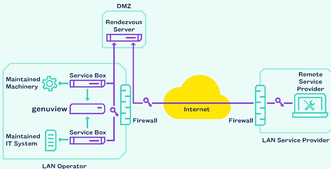
Example showing integration of genuview into a remote-maintenance ecosystem
