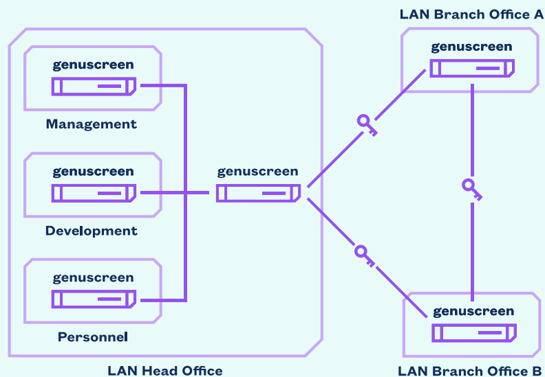
Security zones and encrypted data communication with genuscreen
