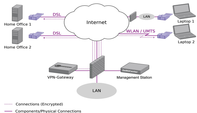
External access to the LAN via VPNs
